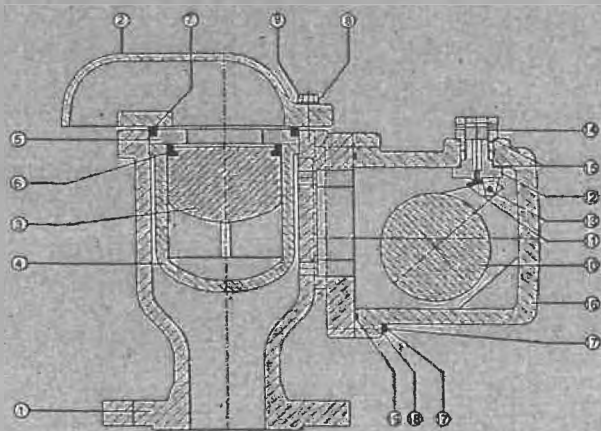
DN 40 – DN 200
